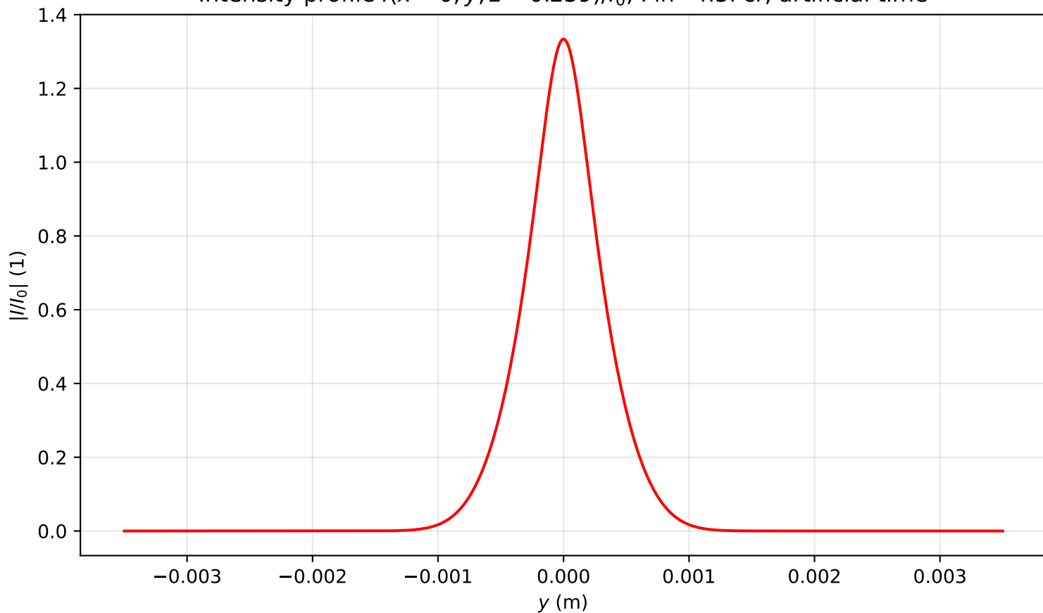
Intensity profile I(x=0, y, z=0.239)/I_0 , P_{in}=4.5P_{cr} , artificial time
